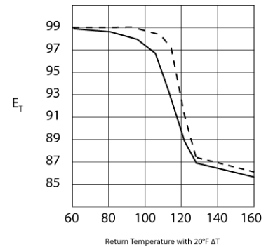
Performance Chart - - - - Low Fire — High Fire
